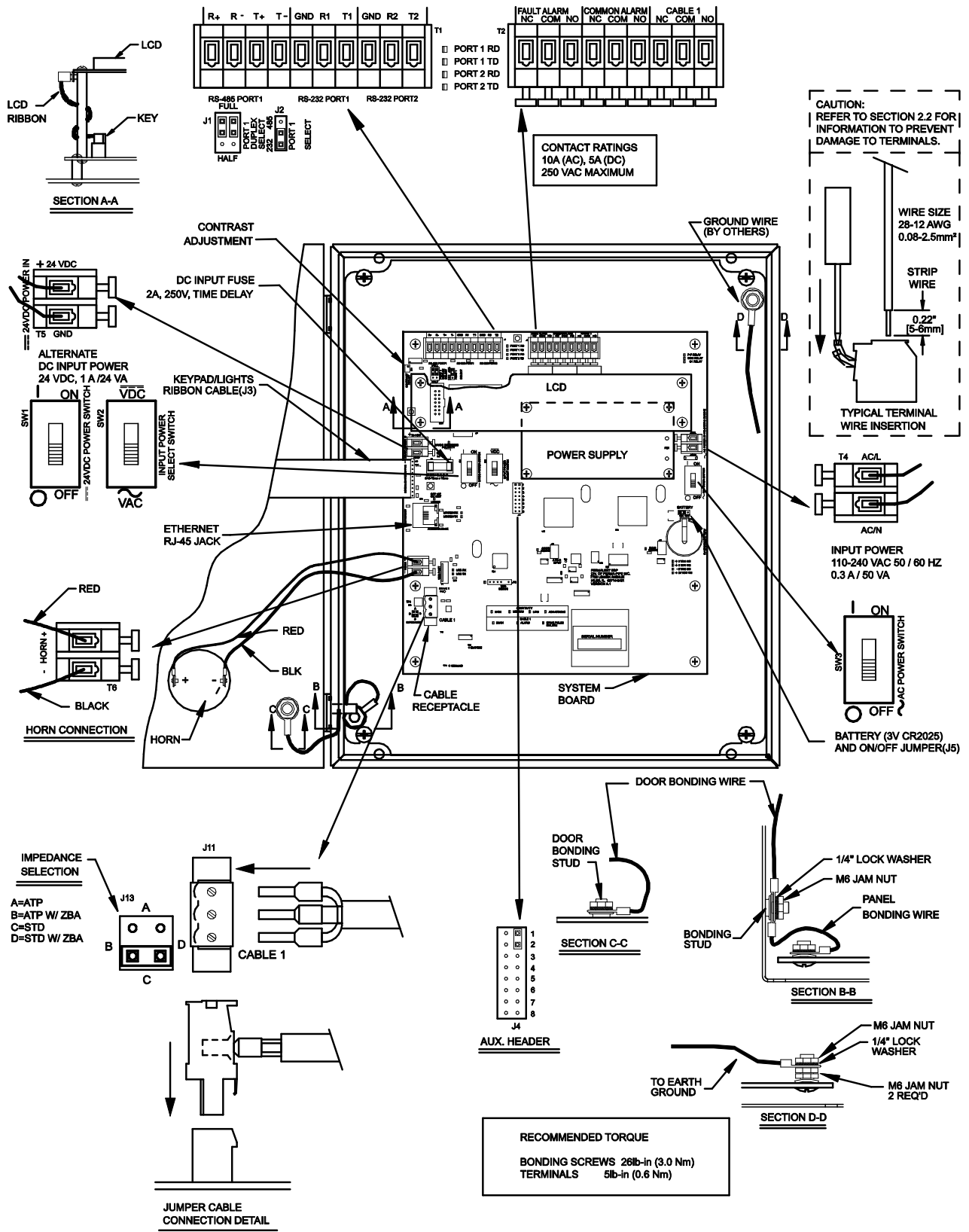
Figure 2-2 Wiring Diagram for PAL-AT Models AT30C & AT75C
