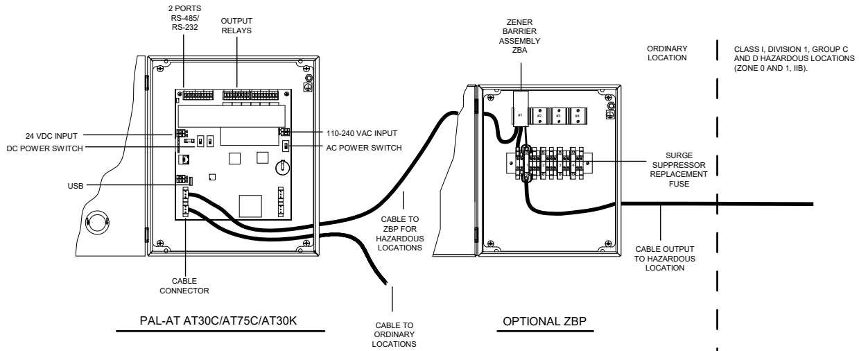
Figure 3-2 PAL-AT and Zener Barrier Panel
