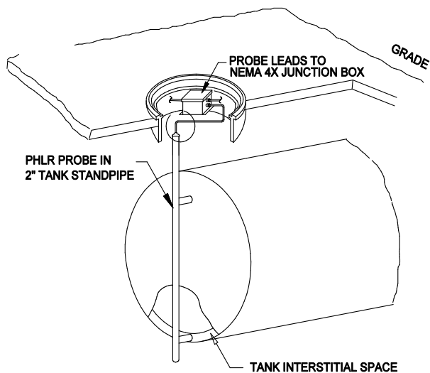
Figure 9-4 Typical PHLR and PHLR-P Probe Installations
